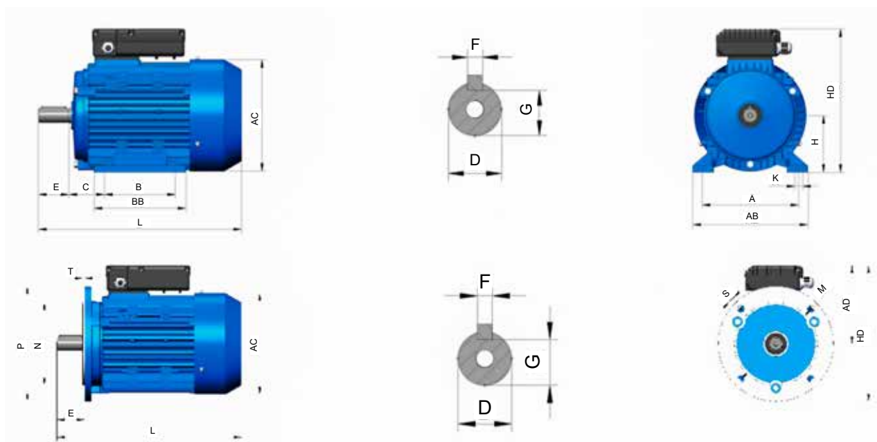
FRAME WITH FEET AND END. SHIELD WITH FLANGE(IM B35)
